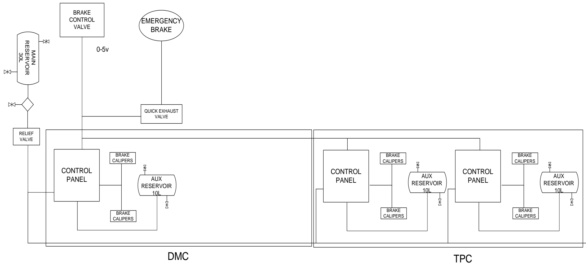
Figure 13: Pneumatic Control Circuit
