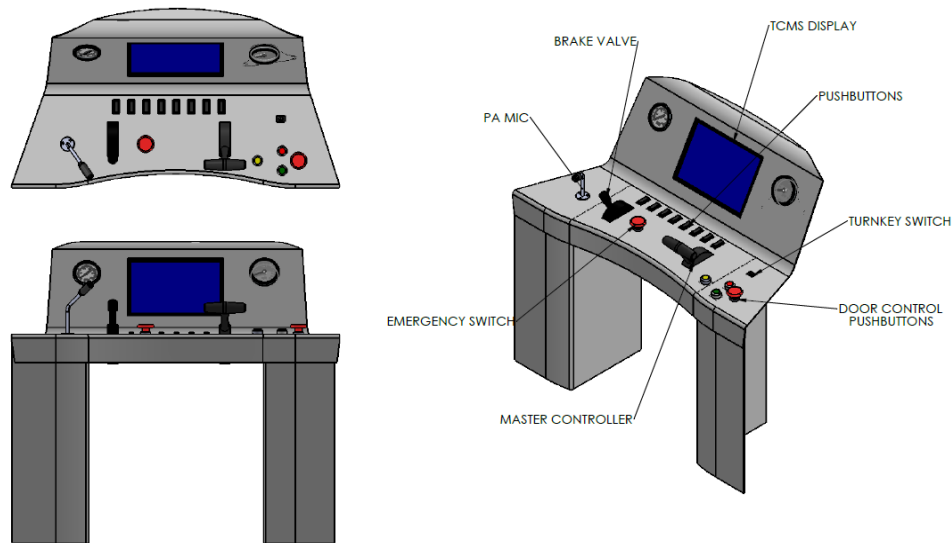
Figure 6: Driver Desk
