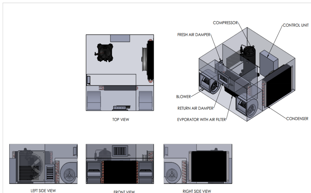
Figure 12: HVAC Unit
