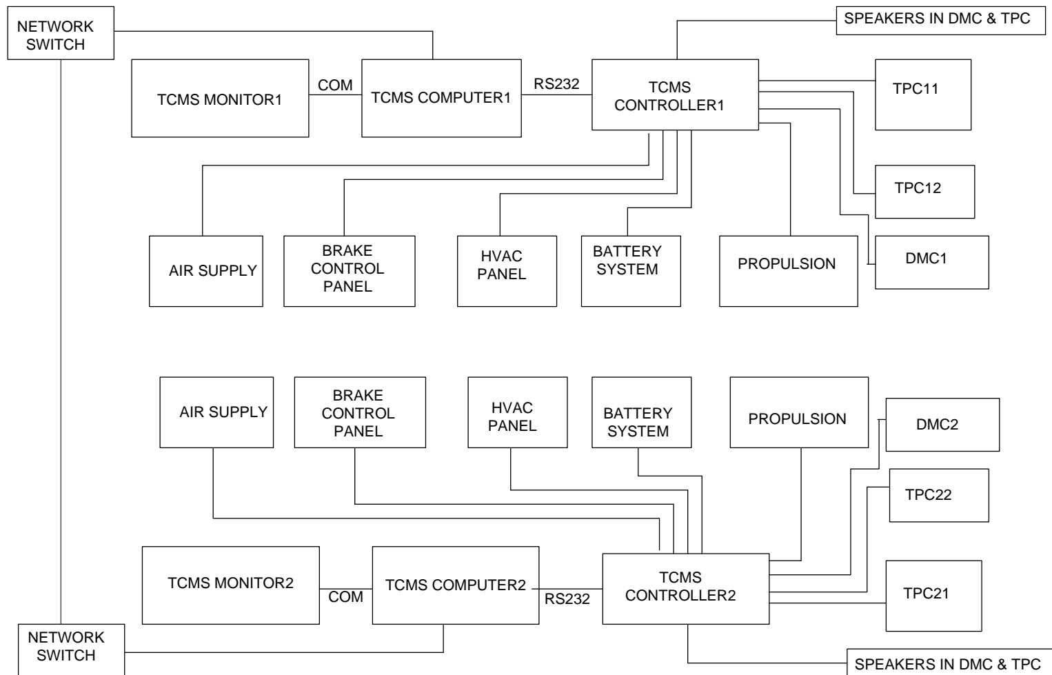
Figure 9: SMBT Communication Network
