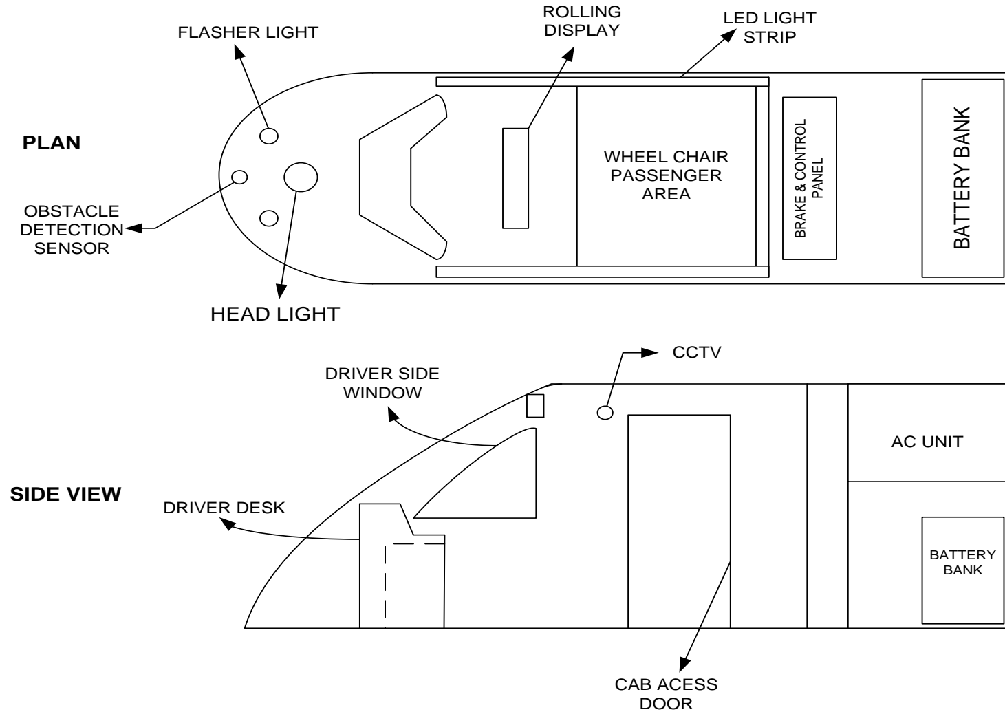
Figure 3: DMC Equipment Location
