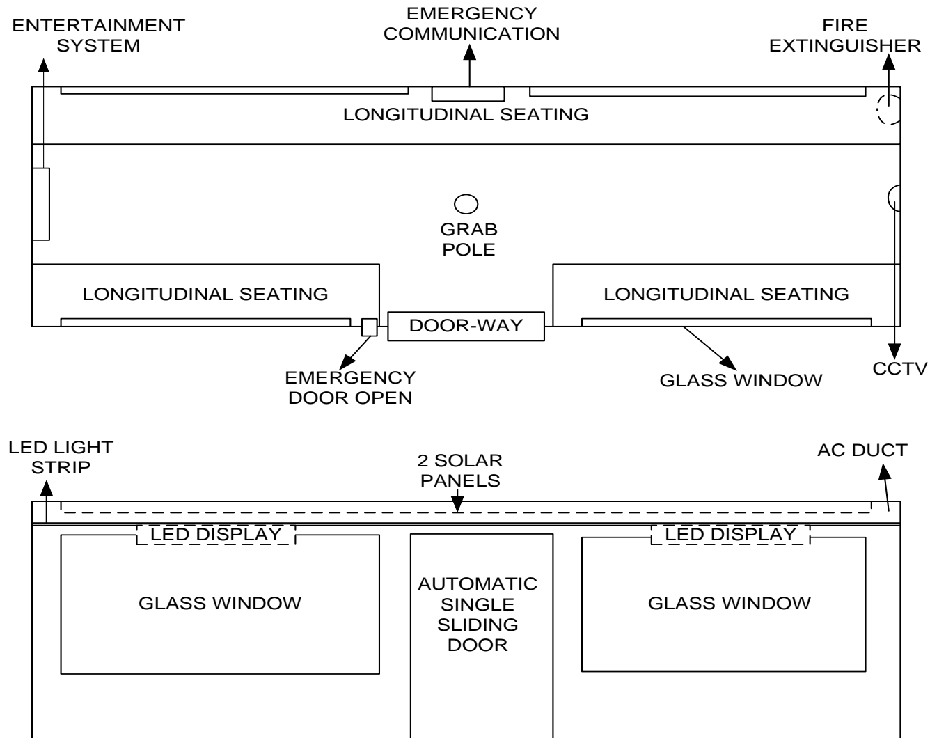
Figure 4: Layout of Equipment in Trailer Car
